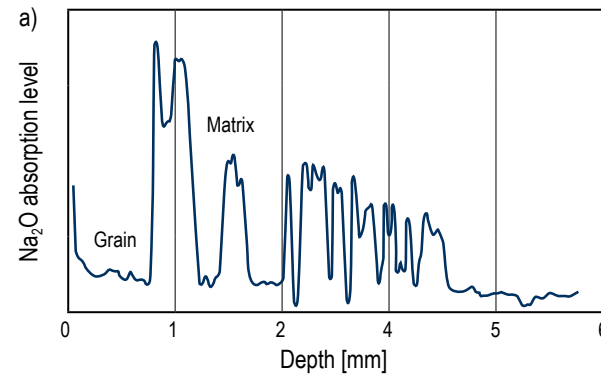
Na 2 O-Absorptionskurve (a) Schamottestein (b) RESISTAL CA65HBL
